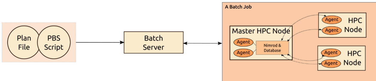
Figure 1: Embedded Nimrod Architecture Diagram
